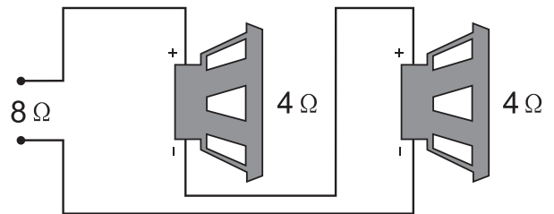
Series wiring
